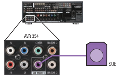
Figure 18 – Subwoofer Connection
